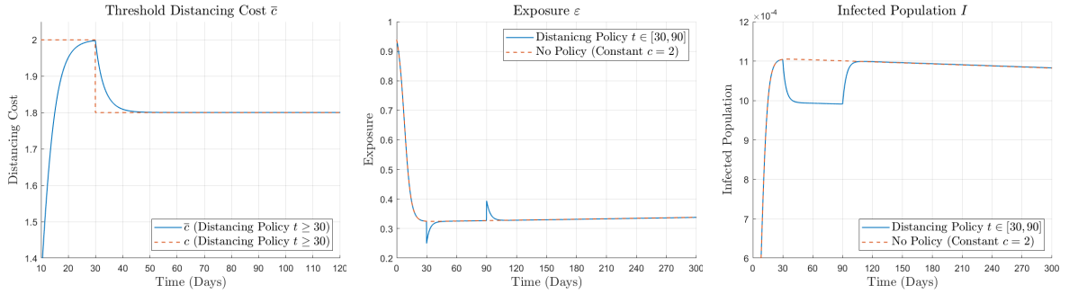
Figure 5: Social-Distancing Policy. The left panel depicts the threshold distancing cost function \bar{c} over time. The central panel depicts the exposure level \varepsilon over time. The right panel depicts the infected population I over time.
