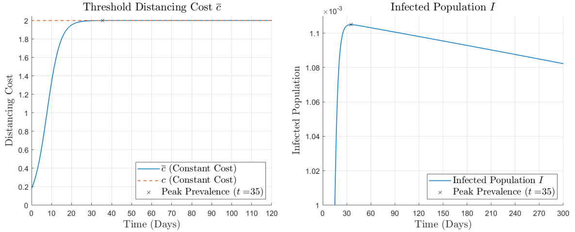
Figure 3: Constant distancing cost. The left panel depicts the threshold distancing cost function \bar{c} over time. The right panel depicts the infected population I over time.
