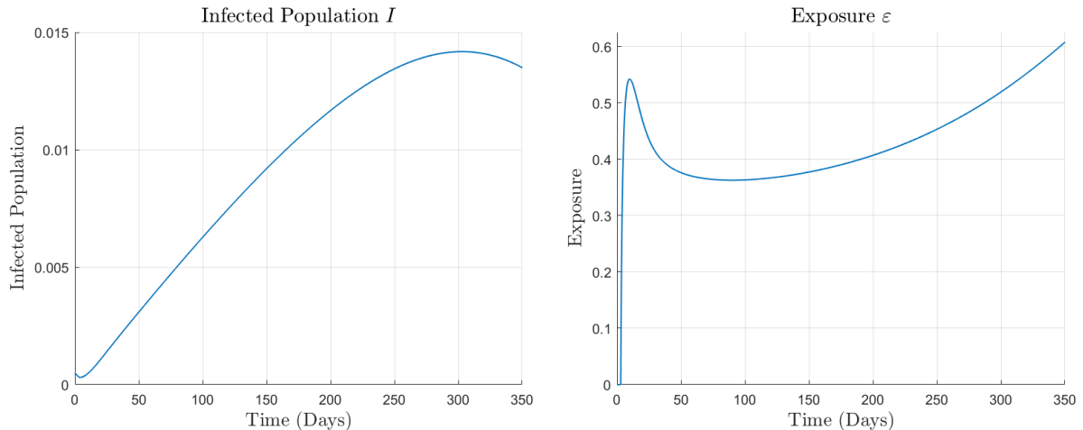
Figure 1: Example 1. The left panel depicts the infected population I over time. While I initially decreases, it starts to increase at around t = 5 . The right panel depicts the exposure level \varepsilon over time.
