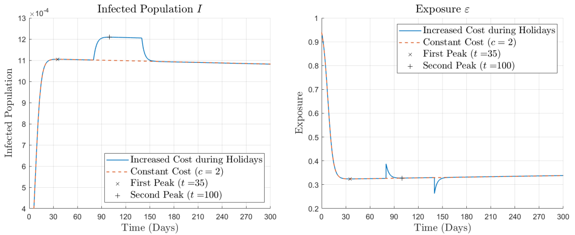
Figure 4: Increased distancing cost during holidays. The left panel depicts the infected population I and especially the second wave. The right panel depicts the exposure level \epsilon .
